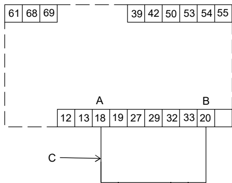
Required minimum connection, signal terminal
