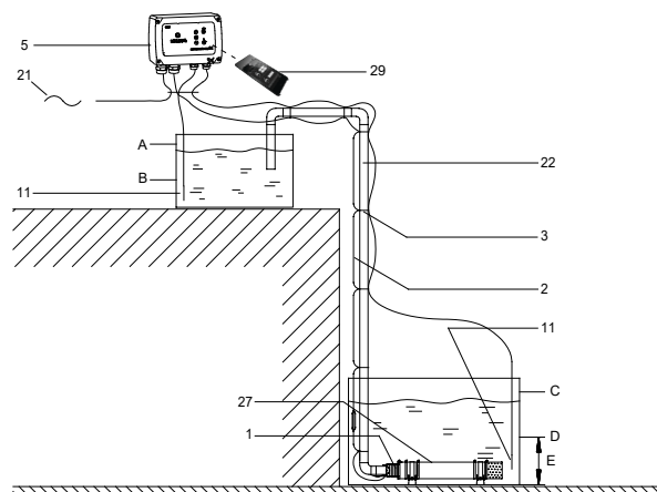
Pumping from one tank to another
