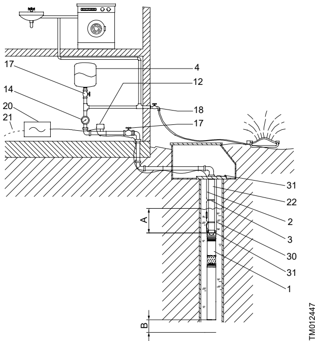
Application example: SQ with pressure switch and pressure tank
