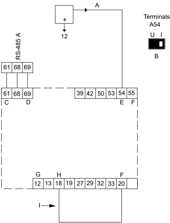
Wiring diagram for SmartFlo
