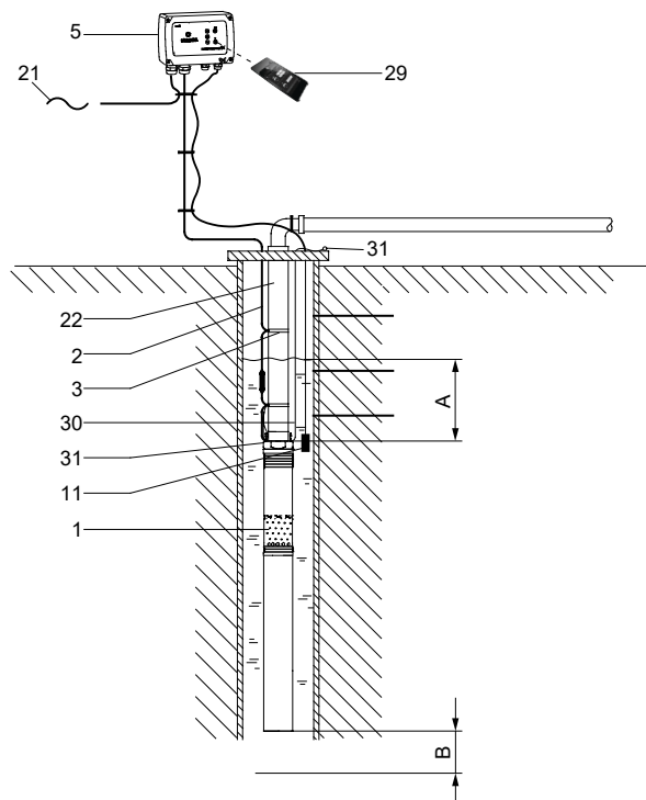
Maintaining a constant water table
